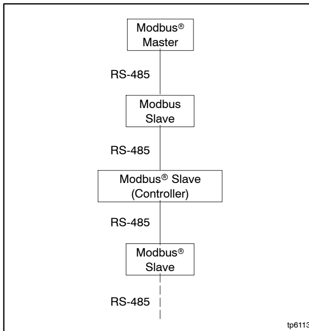
Figure 1-3 RS-485 Network
