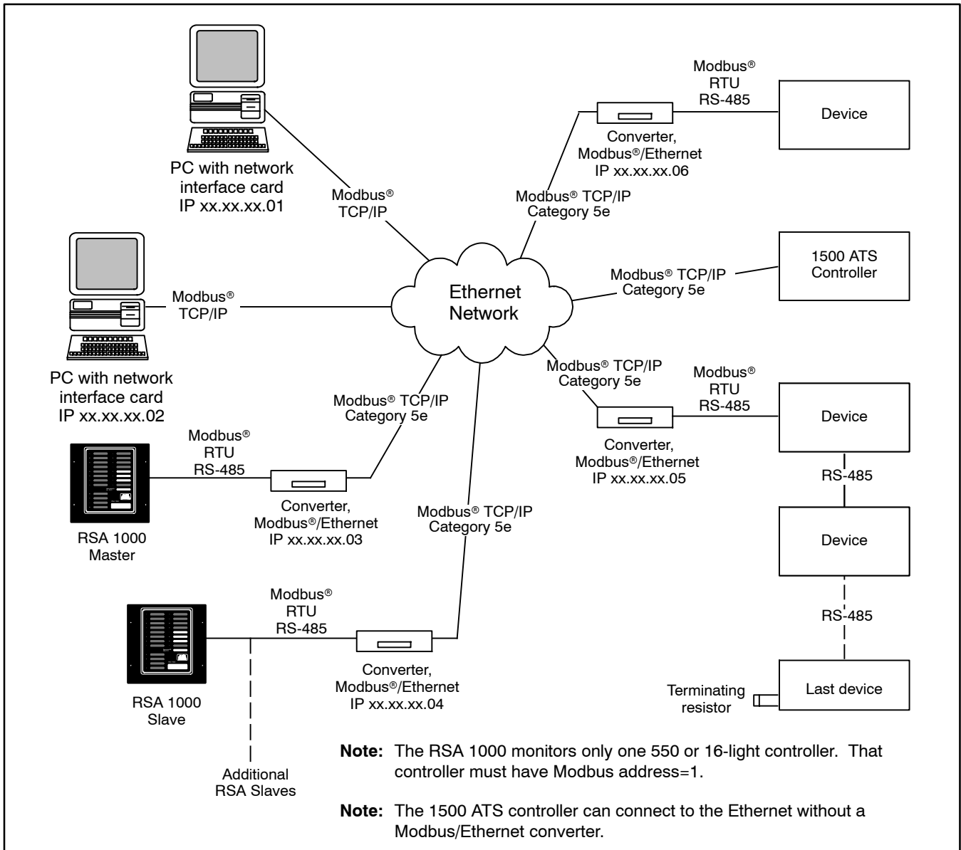
Figure 1-5 Ethernet Connections
