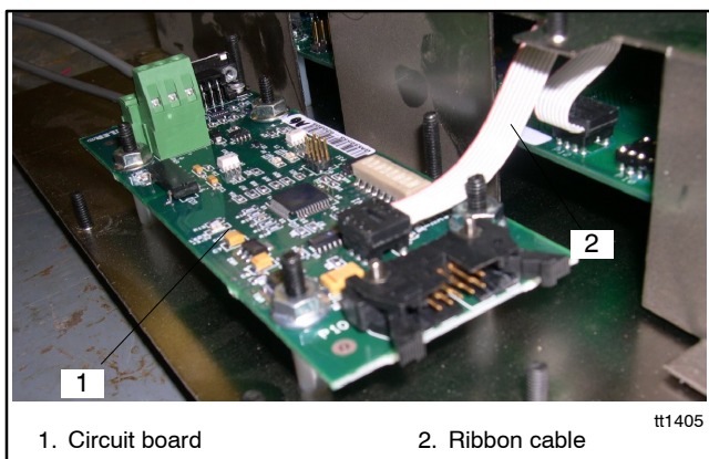
Figure 8-4 Modbus/KBUS Converter Kit, Installed
