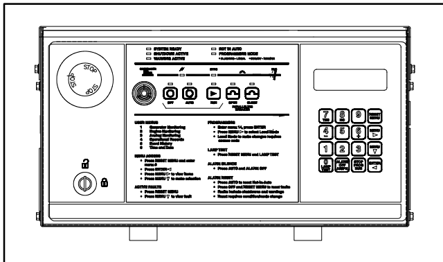
Figure 7-1 Decision-Maker® 6000 Controller
