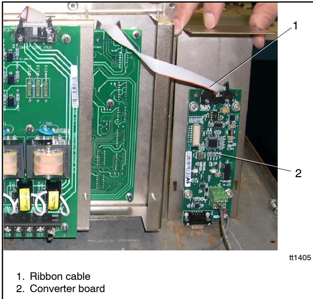
Figure 11-3 Converter Module Location for Power Monitor
