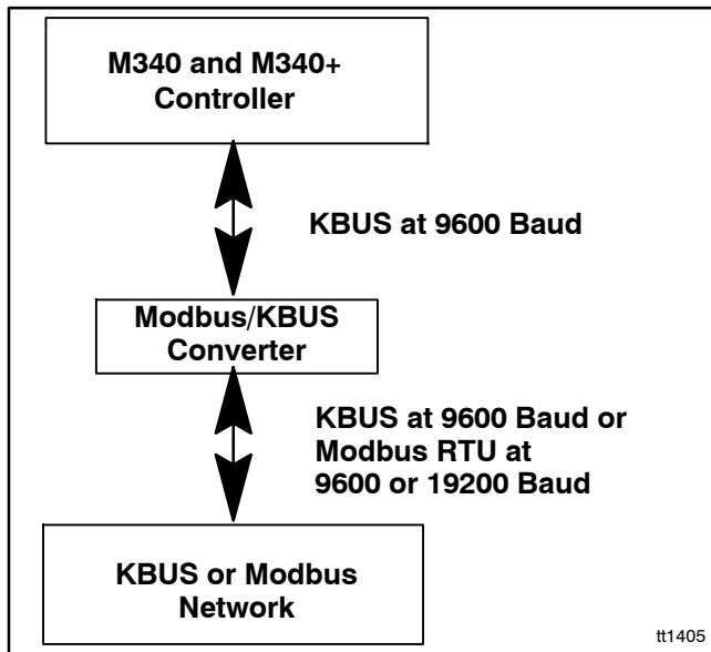
Figure 8-2 Modbus/KBUS Converter Function
