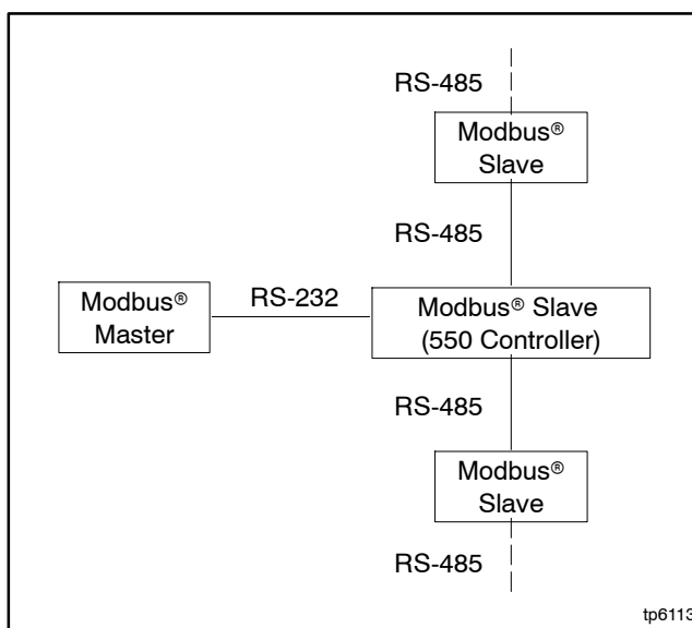
Figure 1-4 RS-485 Network with the 550 Controller used as a Converter
