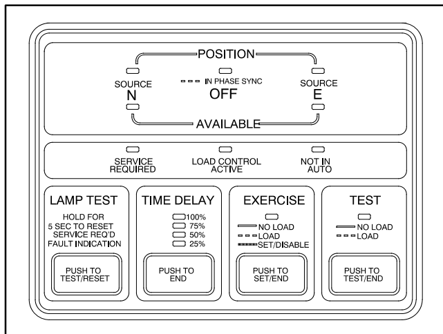
Figure 9-1 MPAC™ 1000 Controller
