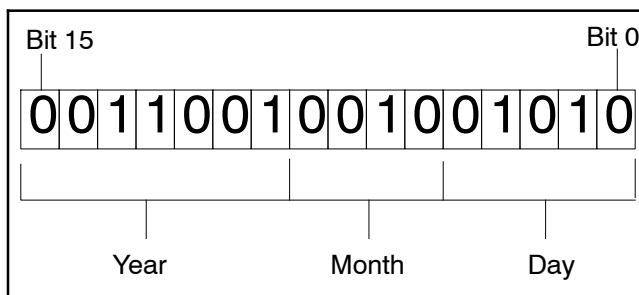
Figure 1-8 16-Bit Word Containing Date 10 February, 2025 (see the example)
