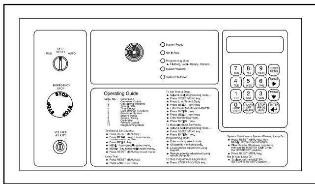
Figure 3-1 Decision-Maker 340 Controller
