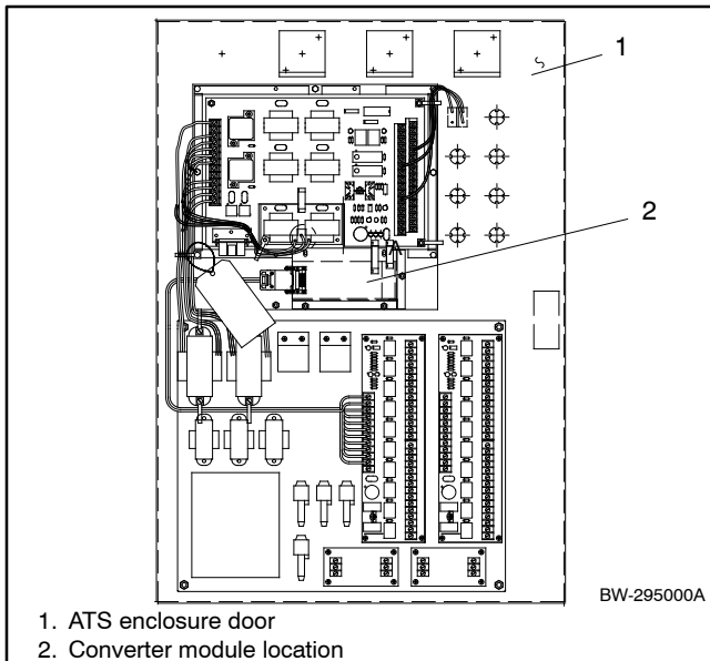
Figure 8-3 Modbus/KBUS Converter Location
