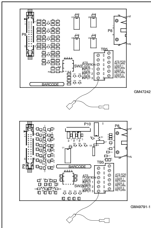
Figure 2-4 Communication Boards
