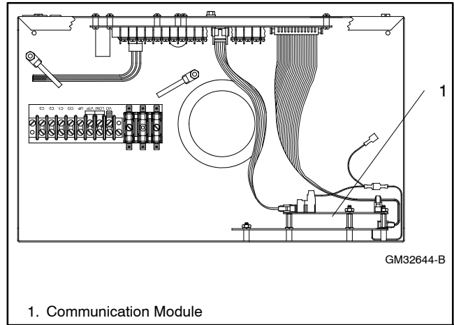
Figure 2-2 Communication Board Location (Controller Top View)
