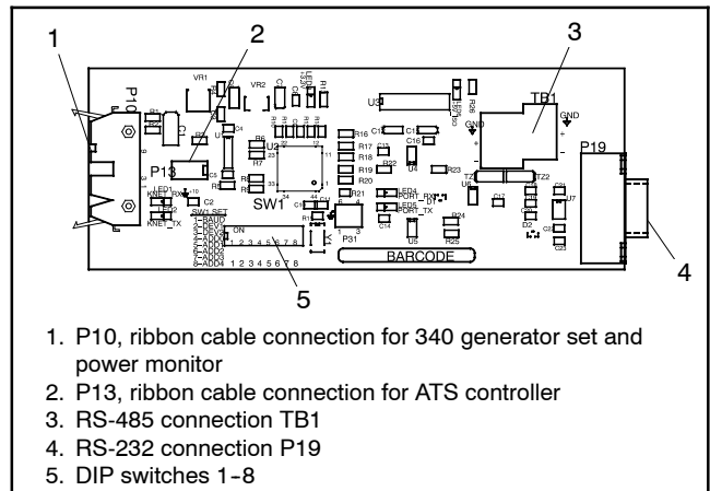
Figure 8-5 Modbus/KBUS Converter Board
