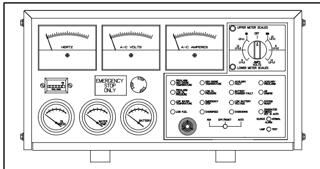
Figure 2-1 Decision-Maker® 3+ Controller
