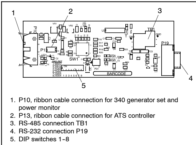
Figure 11-4 Modbus/KBUS Converter Board
