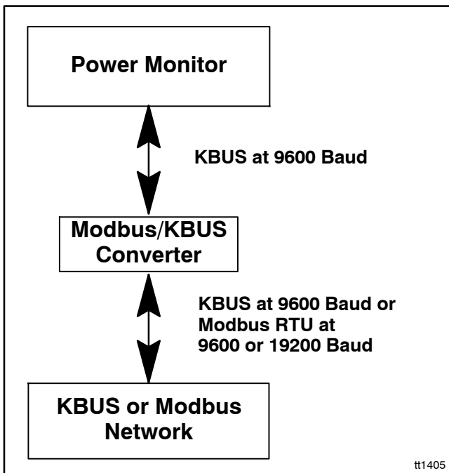
Figure 11-2 Modbus/KBUS Converter Function
