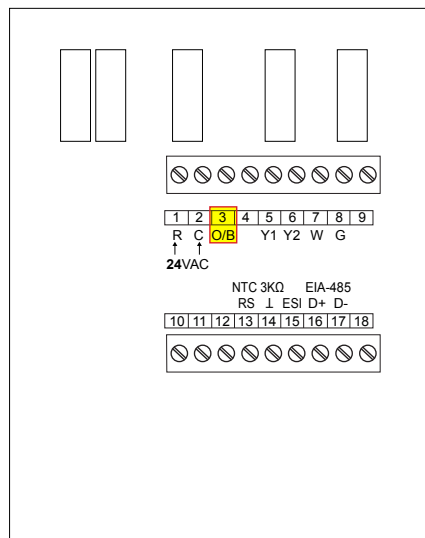
BAST-321HP-B2 and BW2 models
