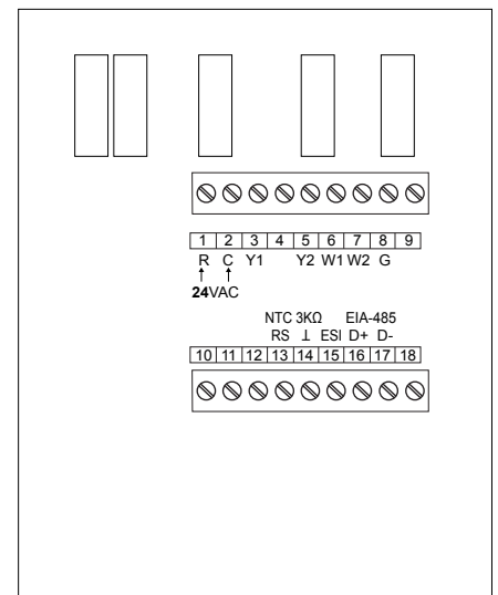
BAST-221C/CH-B2 and BW2 models
