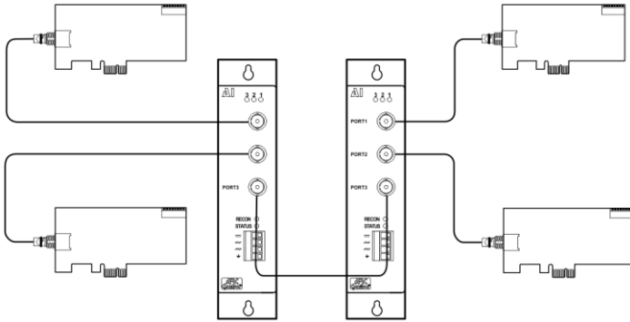
Figure 3 — Point-to-point connections are required between -CXB NIMs and hubs
