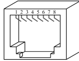
Figure 5 — Modular Jack Numbering Orientation
