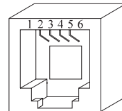
Figure 5—Modular Jack Numbering Orientation
