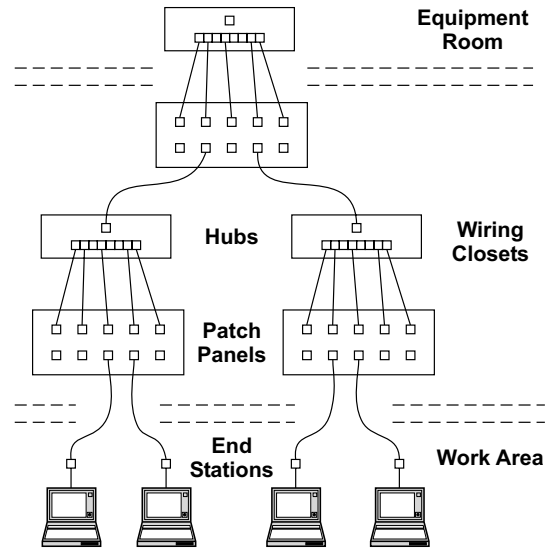
Figure 1. Structured wiring creates a hierarchy of hubs.
